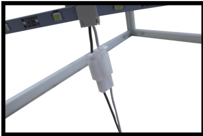
The transformer comes pre wired. Connect wiring from transformer to the 2 plugs at the bottom of the ladder lights.
