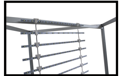
Hang ladder lights from hooks on top cross bar (3ft has 1 light strip, 4ft has 2 strips, 5ft has 3 strips)
