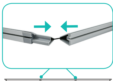
a. Expand each Channel Bars. Follow bungee to connect.
