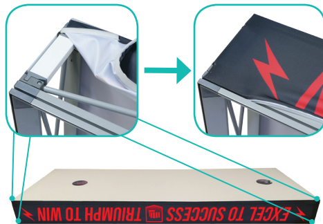
b. Install the end cap graphics on each side of the frame.
