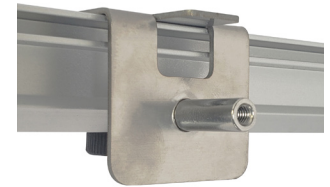
BRIDGE CONNECTION
